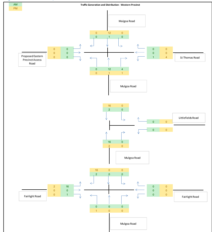
Figure 4.1: Anticipated Western Precinct Traffic Generation and Distribution
