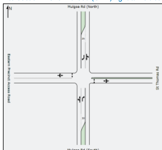
Figure 4.9: Mulgoa Road/St Thomas Road/Eastern Precinct Access Road Intersection – Channelised (CHR) right turns treatment
