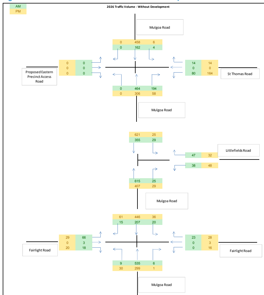
Figure 4.3: 2026 Traffic volumes WITHOUT development
